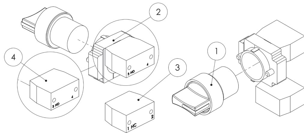
FIGURE 23: Key Switch Subparts
