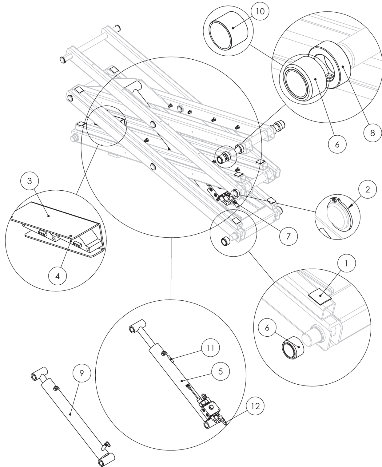
FIGURE 24: Scissors Parts - HB-830
