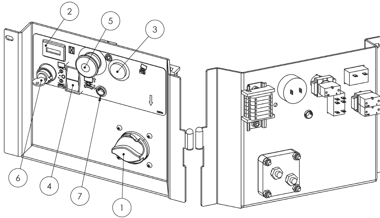
FIGURE 17: Lower Control Parts - ANSI
