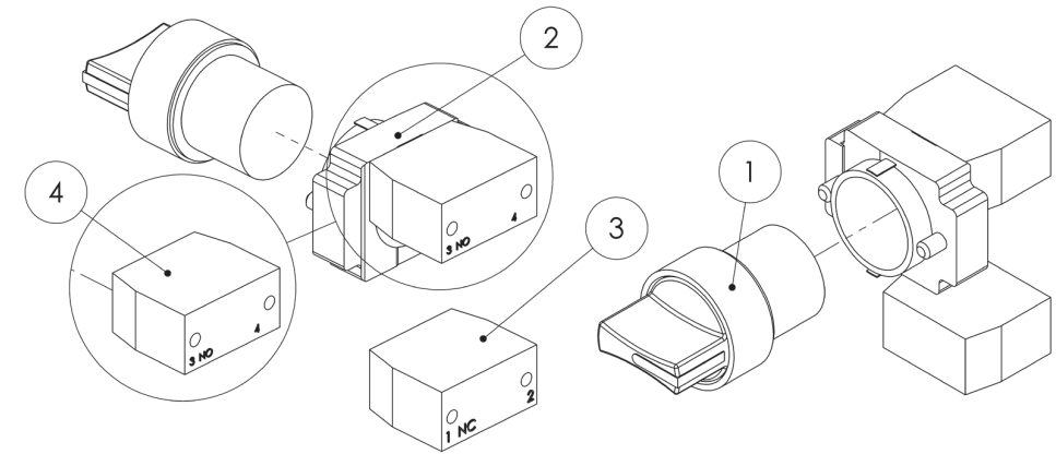
FIGURE 20: Selector Switch Subparts
