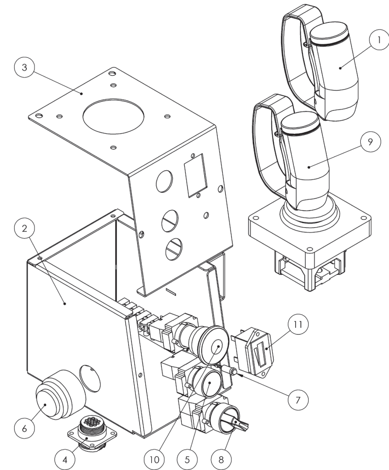
FIGURE 16: Upper Control Parts - CE
