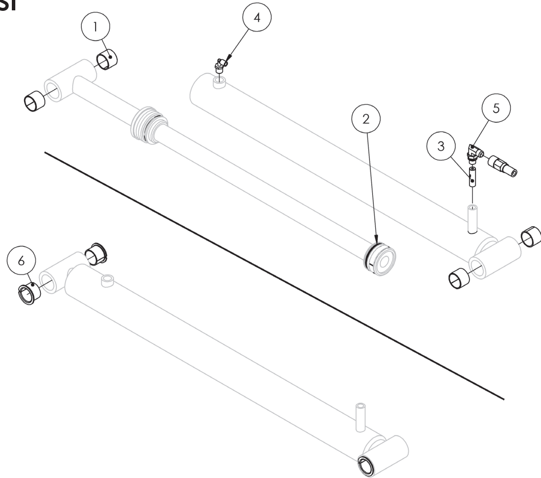
FIGURE 26: Cylinder Subparts - ANSI
