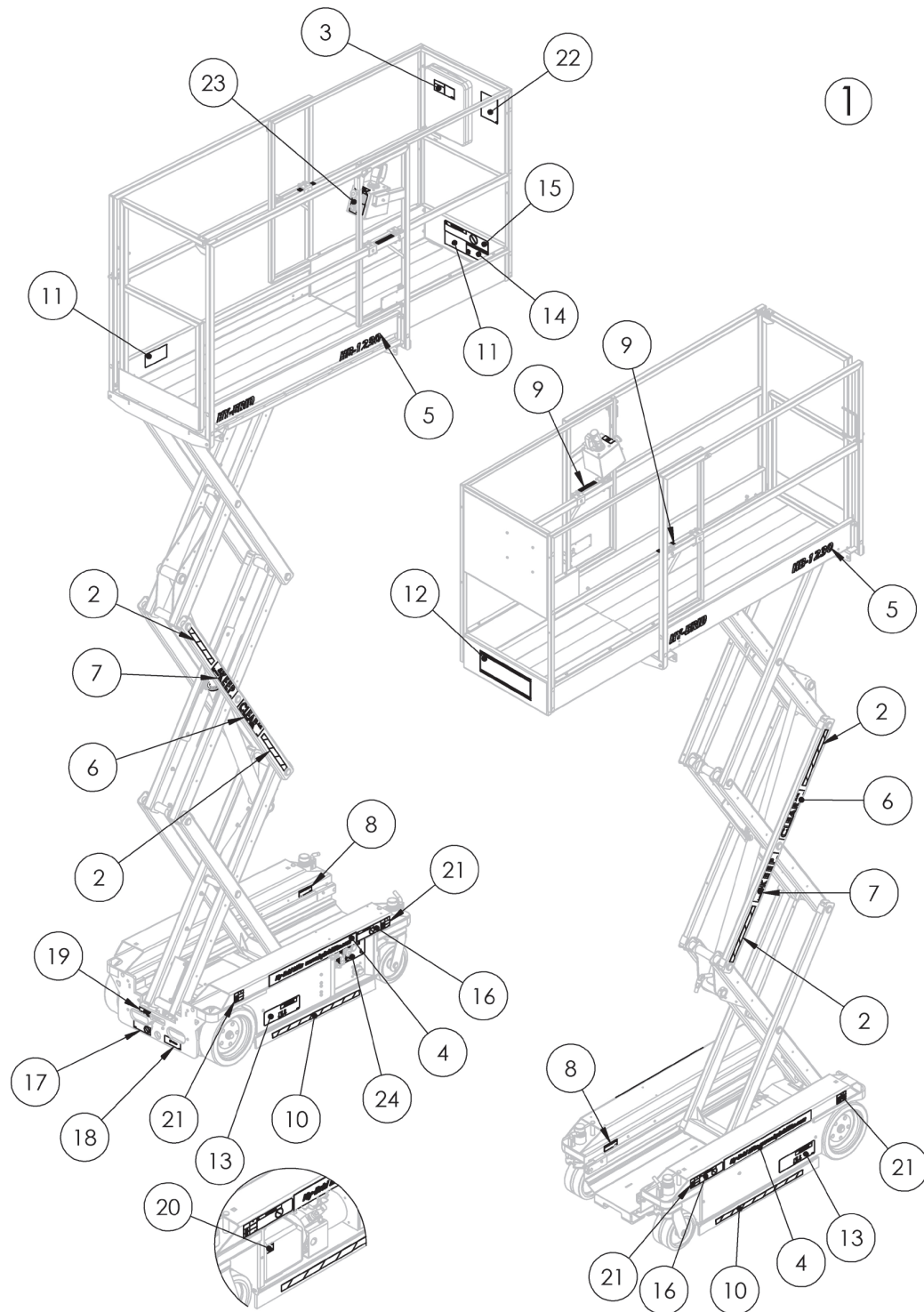
FIGURE 29: Decals - HB-1230 - ANSI
