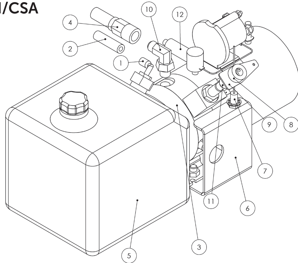
FIGURE 8: Pump Parts - ANSI/CSA
