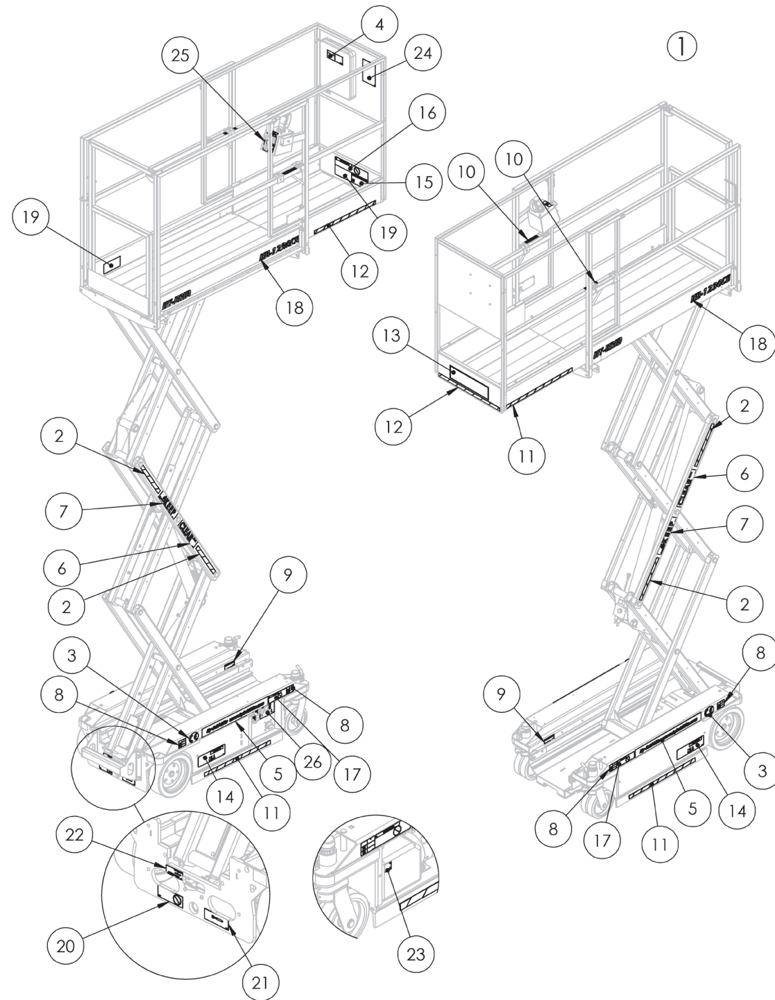
FIGURE 30: Decals - HB-1230 - CE
