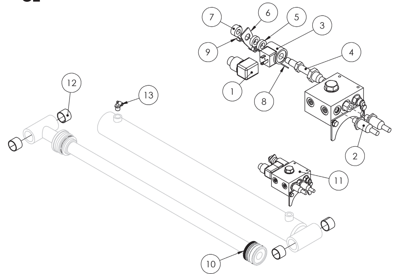
FIGURE 27: Cylinder Subparts - CE
