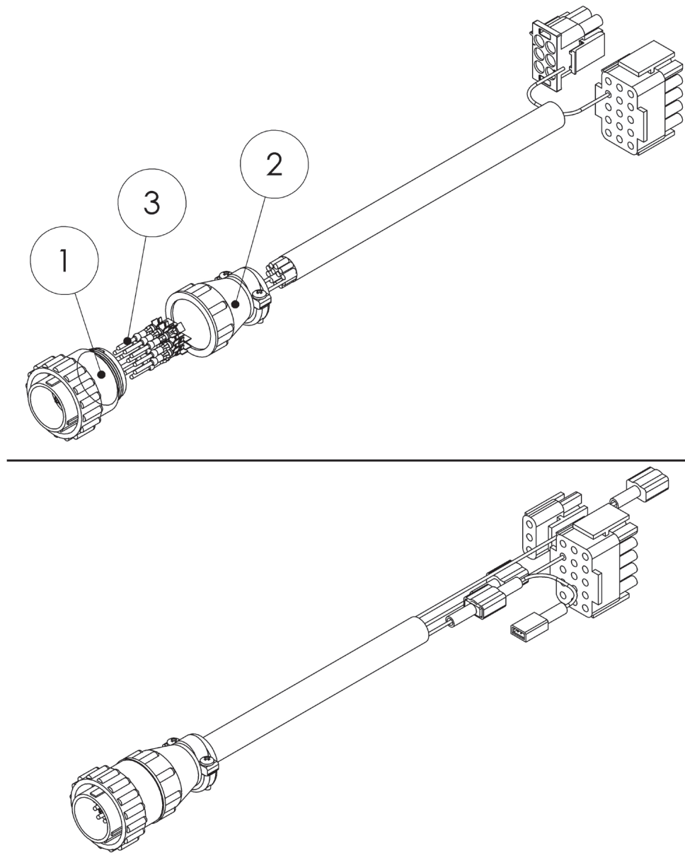
FIGURE 19: Main Cable Subparts
