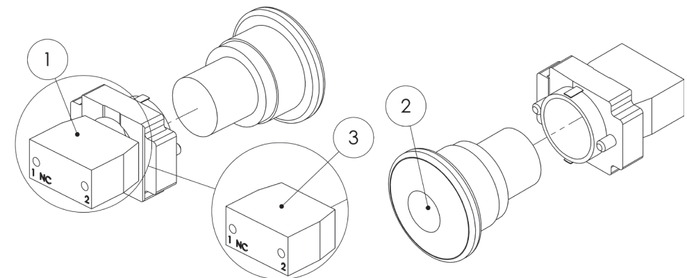
FIGURE 21: E-Stop Switch Subparts
