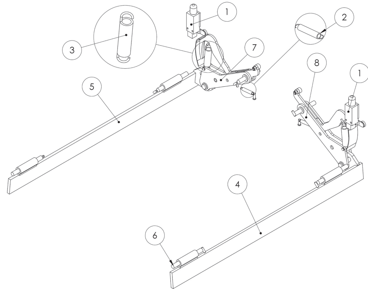
FIGURE 1: Pothole Guard Parts
