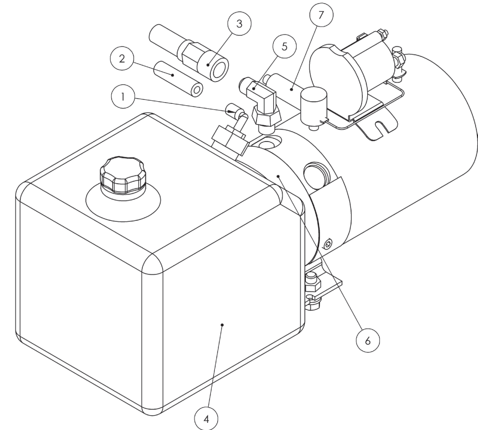
FIGURE 9: Pump Parts - CE
