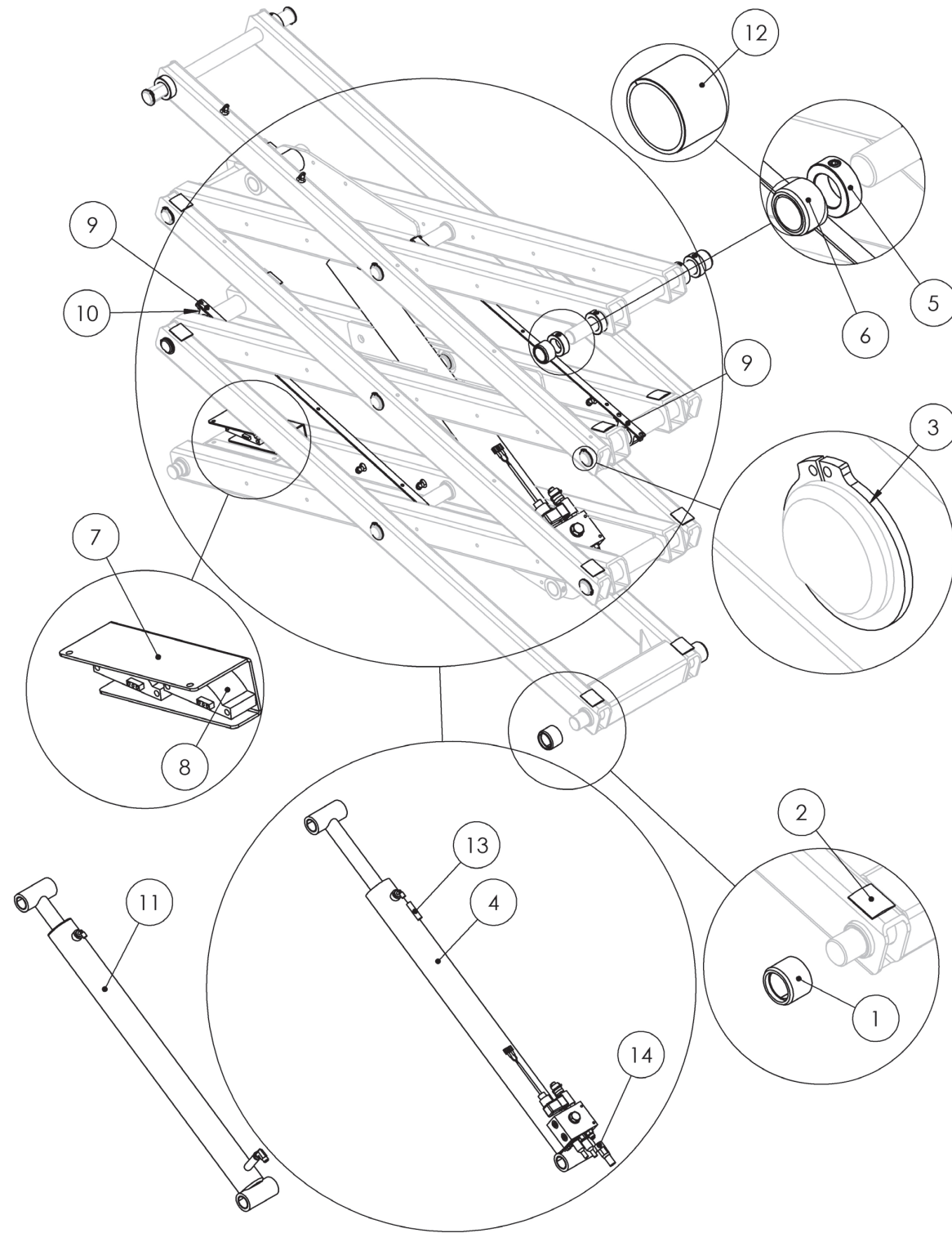
FIGURE 25: Scissors Parts - HB-1230
