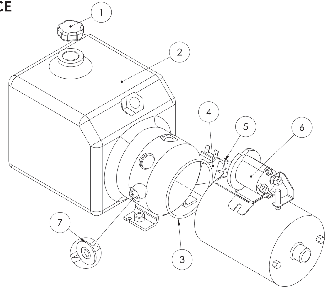
FIGURE 11: Pump Subparts - CE
